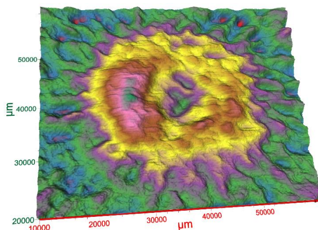
Fig. 2. A drop of Nano cellulose solution on a silicon wafer dried at room temperature. The image was generated by a camera less T-ray nanoscanning technique [5].
